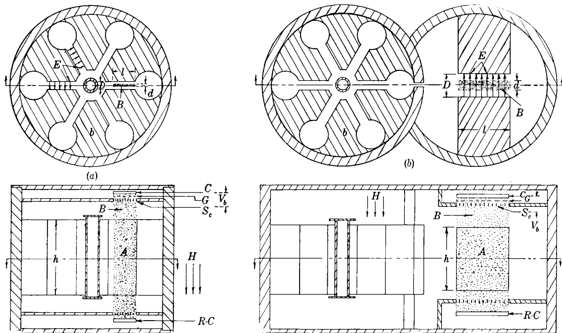
FIG. 15-1.—Examples of electronic tuning of magnetrons. (a) Internal tuning. H is the d-c magnetic field; B is the electron beam; l is the beam length; d is the beam width; \bar{E} is the r-f electric field; D is the gap width; \bar{E}D is the r-f voltage \bar{V}_{RF} ; h is the condenser plate height; A is the condenser area lh traversed by the beam; AD is the gap region traversed by the beam; Ad is the beam region; C is the cathode for the electron beam; G is the control grid; S_e is the screen grid; R-C is the reflector or collector; V_b is the cathode-to-screen-grid voltage, which equals the cathode-to-condenser plate voltage; and b is the copper block. (b) External tuning, showing the magnetron and reactance tube.
